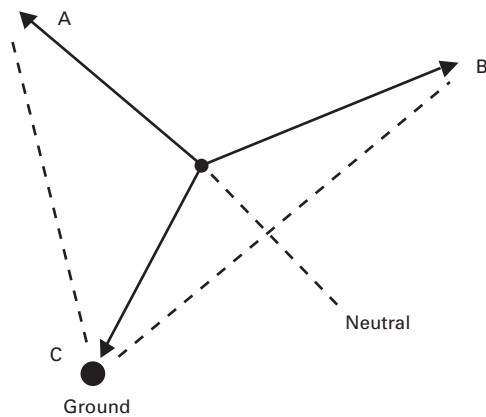
FIGURE 7. PHASE C FAULT CONDITION
