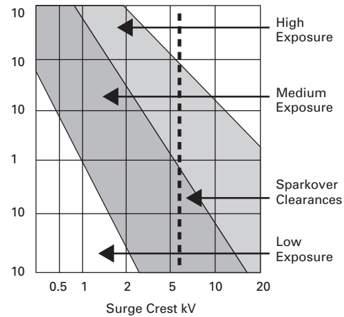
FIGURE 4. IEEE C62.41 EXPOSURE LEVELS
