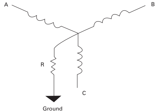
FIGURE 5. RESISTANCE GROUNDING SCHEME
