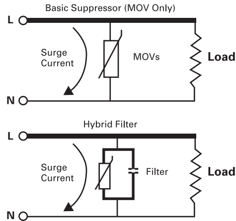
FIGURE 10. BASIC SUPPRESSOR AND HYBRID FILTER
