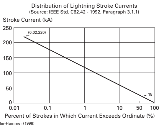
FIGURE 9. DISTRIBUTION OF LIGHTNING STROKE CURRENTS
