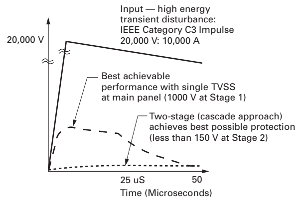
FIGURE 8. FACILITY-WIDE PROTECTION SOLUTIONS — IEEE EMERALD BOOK RECOMMENDS A CASCADE (OR 2-STAGE) APPROACH
