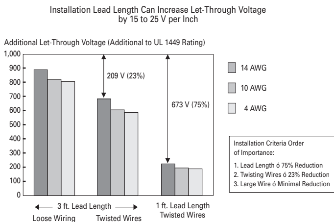
FIGURE 17. ADDITIONAL LET-THROUGH VOLTAGE USING IEEE C1 (6000V, 3000A) WAVEFORM (UL1449 TEST WAVE)
