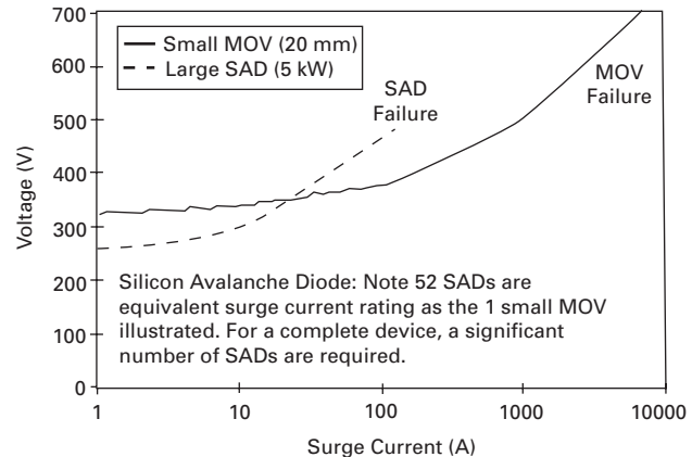
FIGURE 13. SILICON AVALANCHE DIODES HAVE LIMITED ENERGY CAPABILITY
