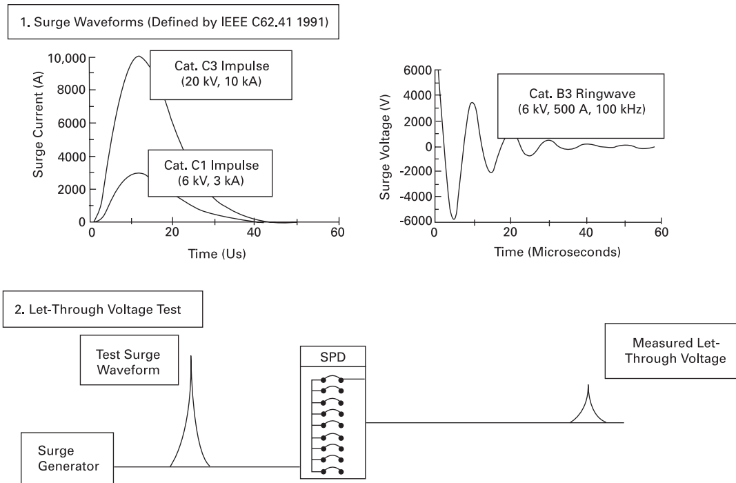
FIGURE 16. EXAMPLE OF LET-THROUGH VOLTAGES AND DIFFERENT IEEE DEFINED SURGE WAVEFORMS
