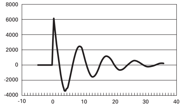
FIGURE 2. RINGWAVE
