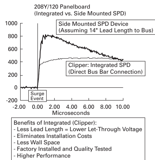
FIGURE 18. INTEGRATED SPD PERFORMANCE
