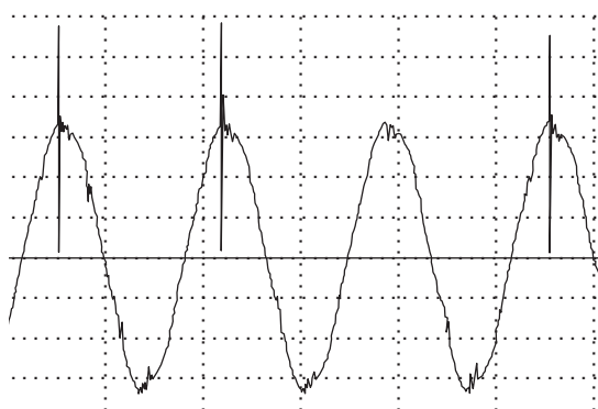
FIGURE 20. EMI/RFI ELECTRICAL LINE NOISE
