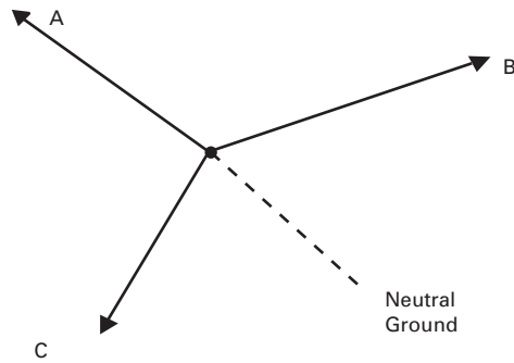
FIGURE 6. WYE SYSTEM
