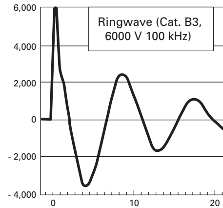
FIGURE 11. RINGWAVE
