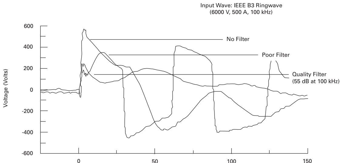
FIGURE 12. RINGWAVE SUPPRESSION CAPABILITIES
